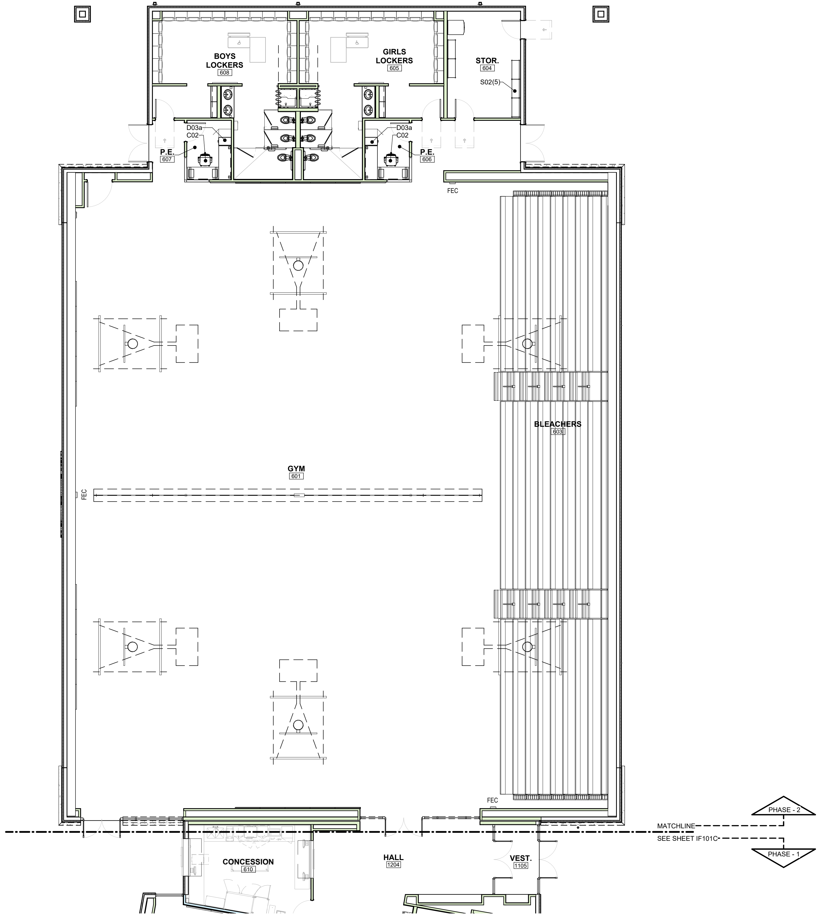
A1 FURNITURE PLAN - AREA D 1/8" = 1'-0"
