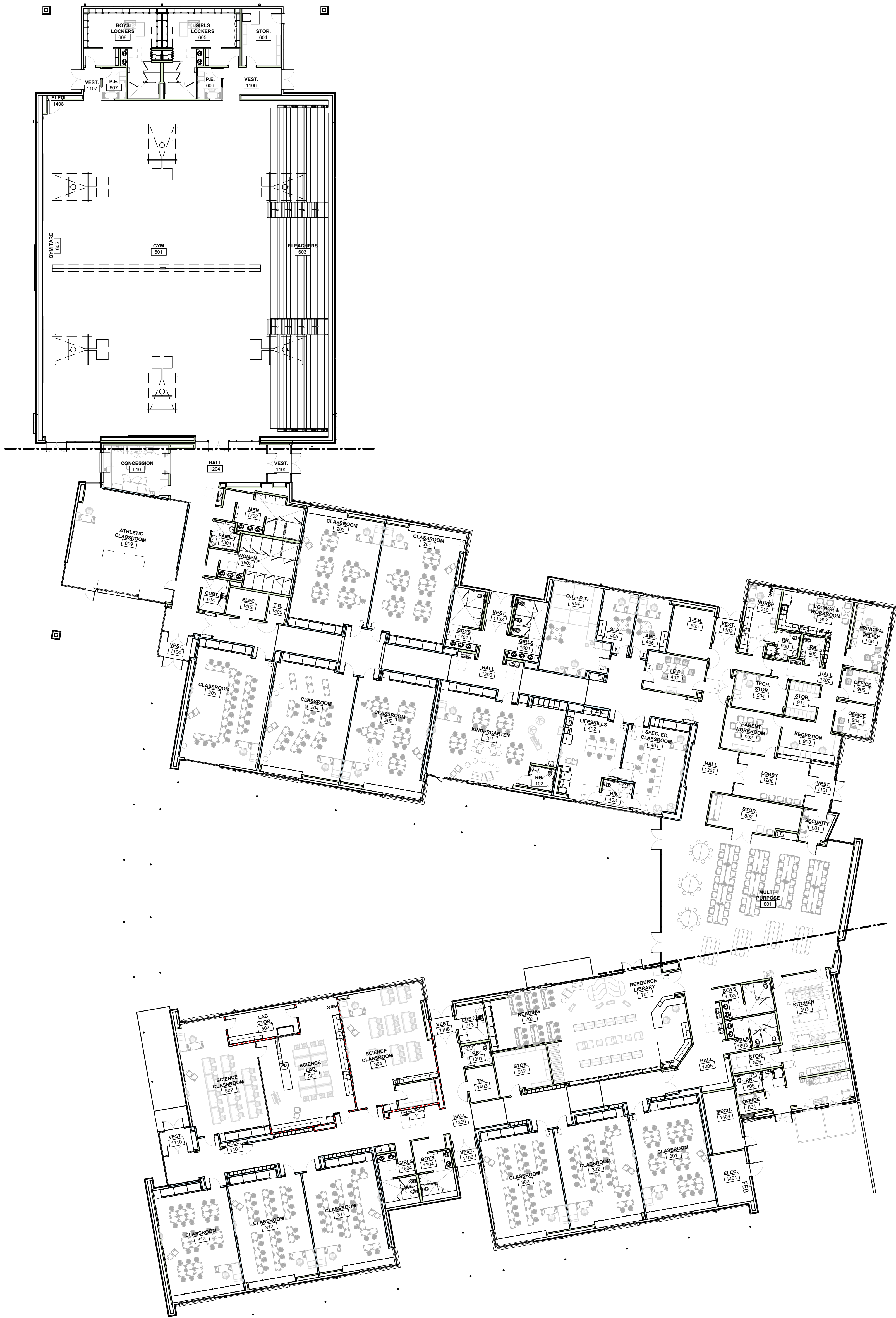
A4 FURNITURE PLAN 1/16" = 1'-0"
